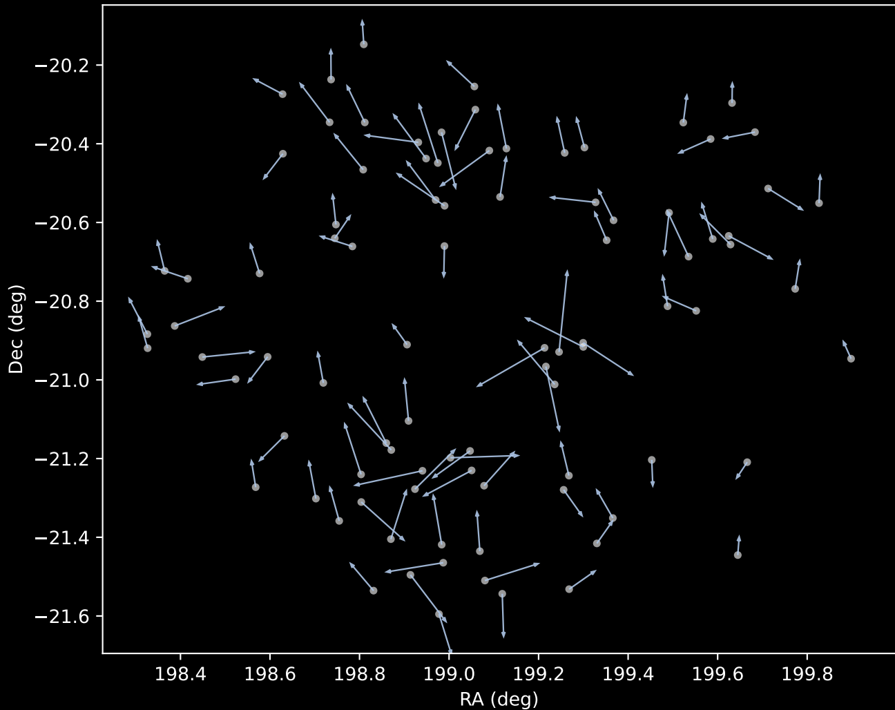
GALAH DR4 Cluster 1 Proper Motion Vectors (n=91)
